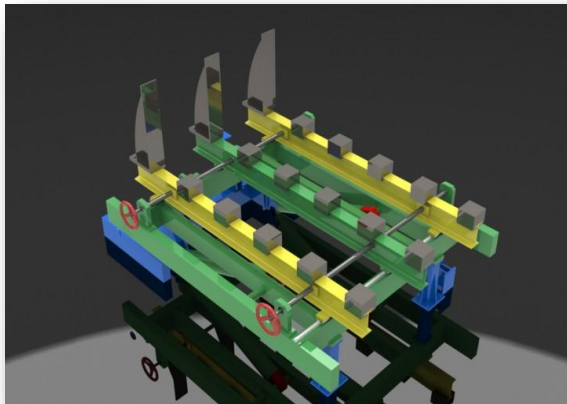
Core Tilting Table
