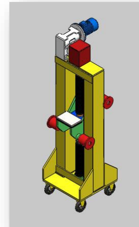
Synchronized Screw Jack
