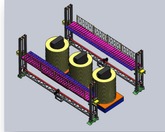
Active Part Assly. Platform
