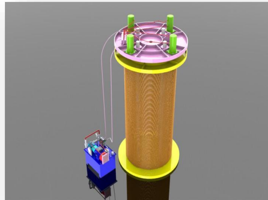
Coil Pressing Fixture
