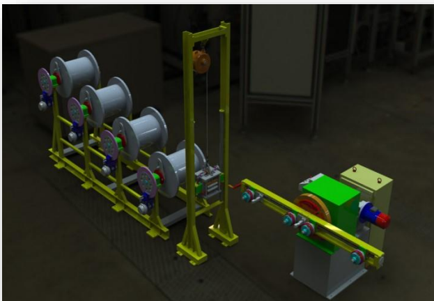
Loop Winding Machine
